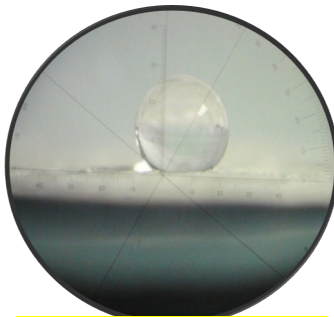
A droplet of water on water resistant paper
